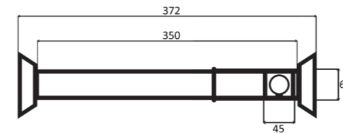
MGL 1x26W STANDART
