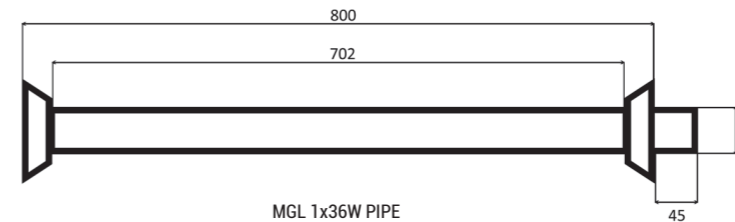
MGL 1x36W PIPE
